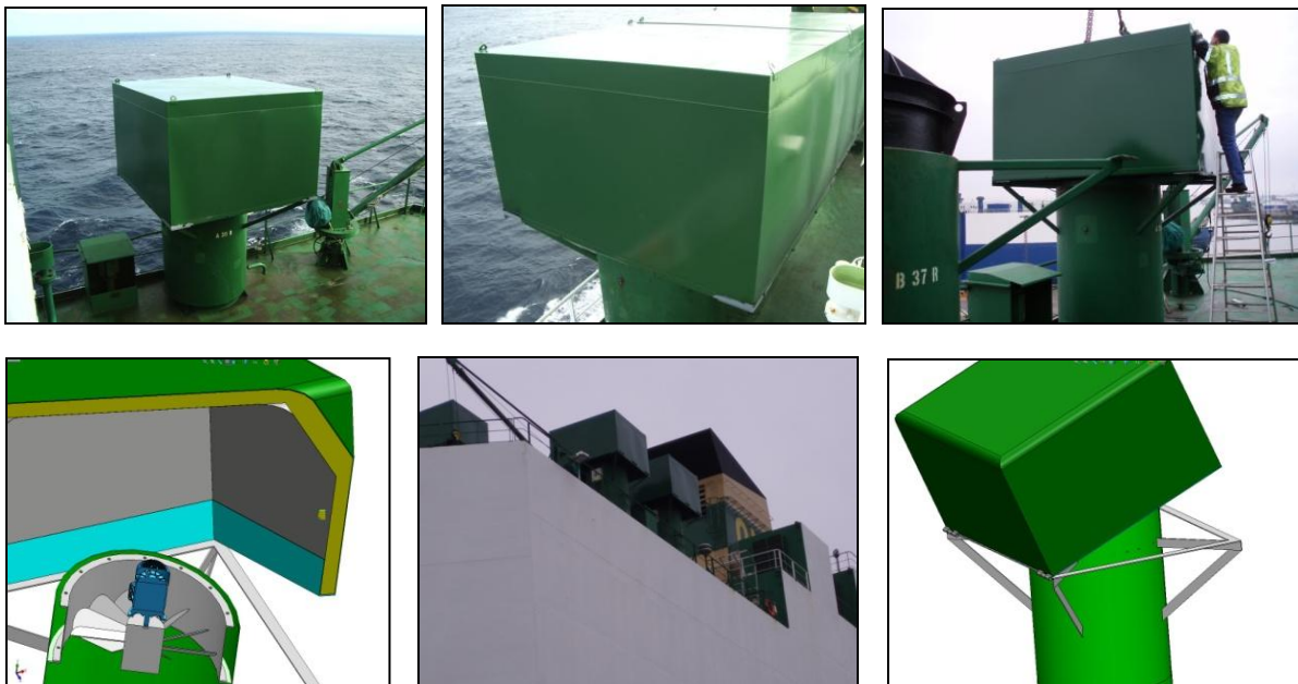
Ventilation hood model. SQ
