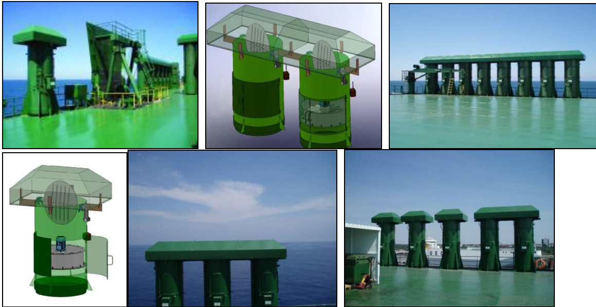
Ventilation hood model. 45
